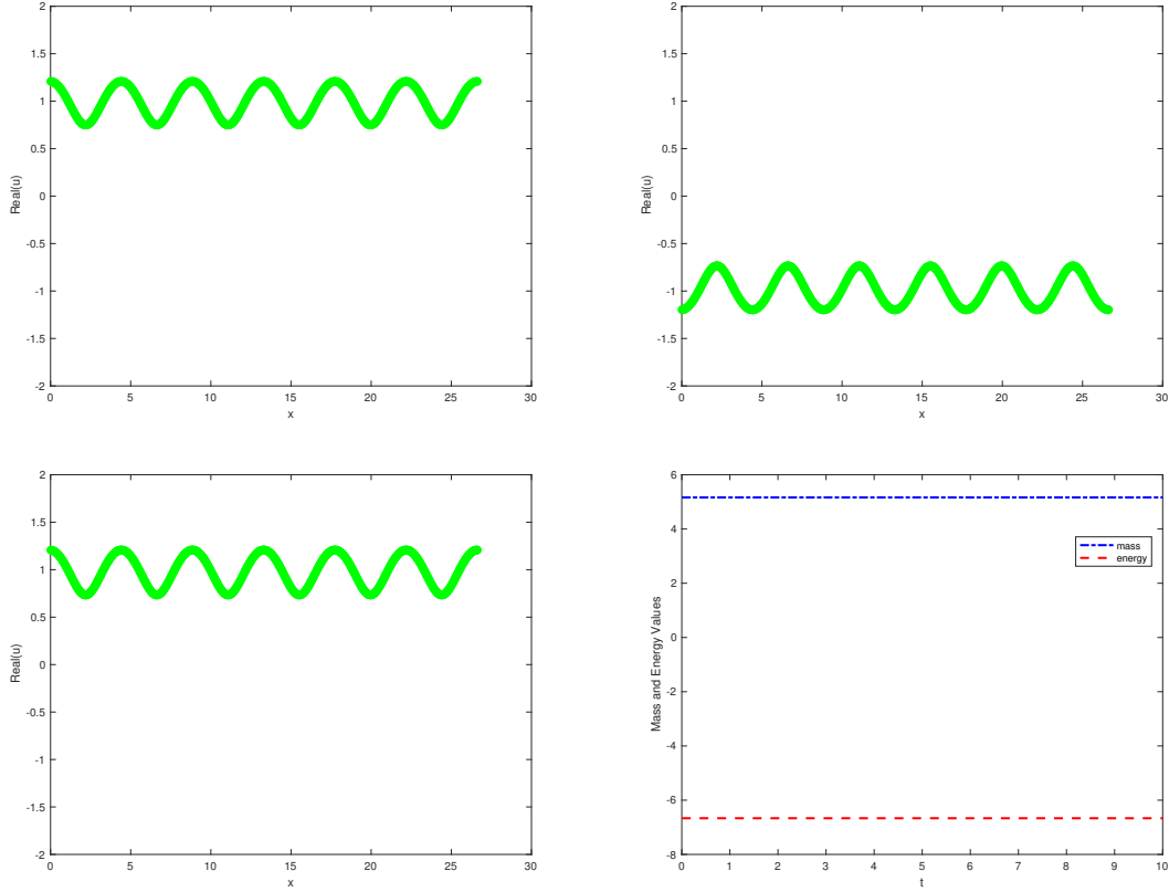
FIGURE 3. Snapshots of the real part of solution of regularized (5.1) with stationary periodic solutions ( v = 0 , c = 1 , B = -.2 ) initial data at time t = 0 (top left), time t = \pi (top right), and time t = 2\pi (bottom left). Also, we plot the Mass and Hamiltonian energy over time (bottom right).
